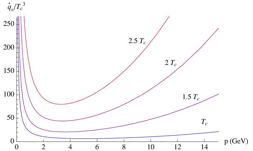
\hat{q}_\parallel charm
