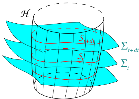
Figure: E. Gourgoulhon, J.L. Jaramillo, Phys.Rept. 423 (2006) 159
